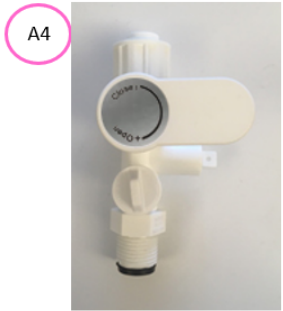
FILTER VALVE 3 IN 1-WH (P) DOME (PLASTIC SHAFT) DOME MESH FILTER WITH
