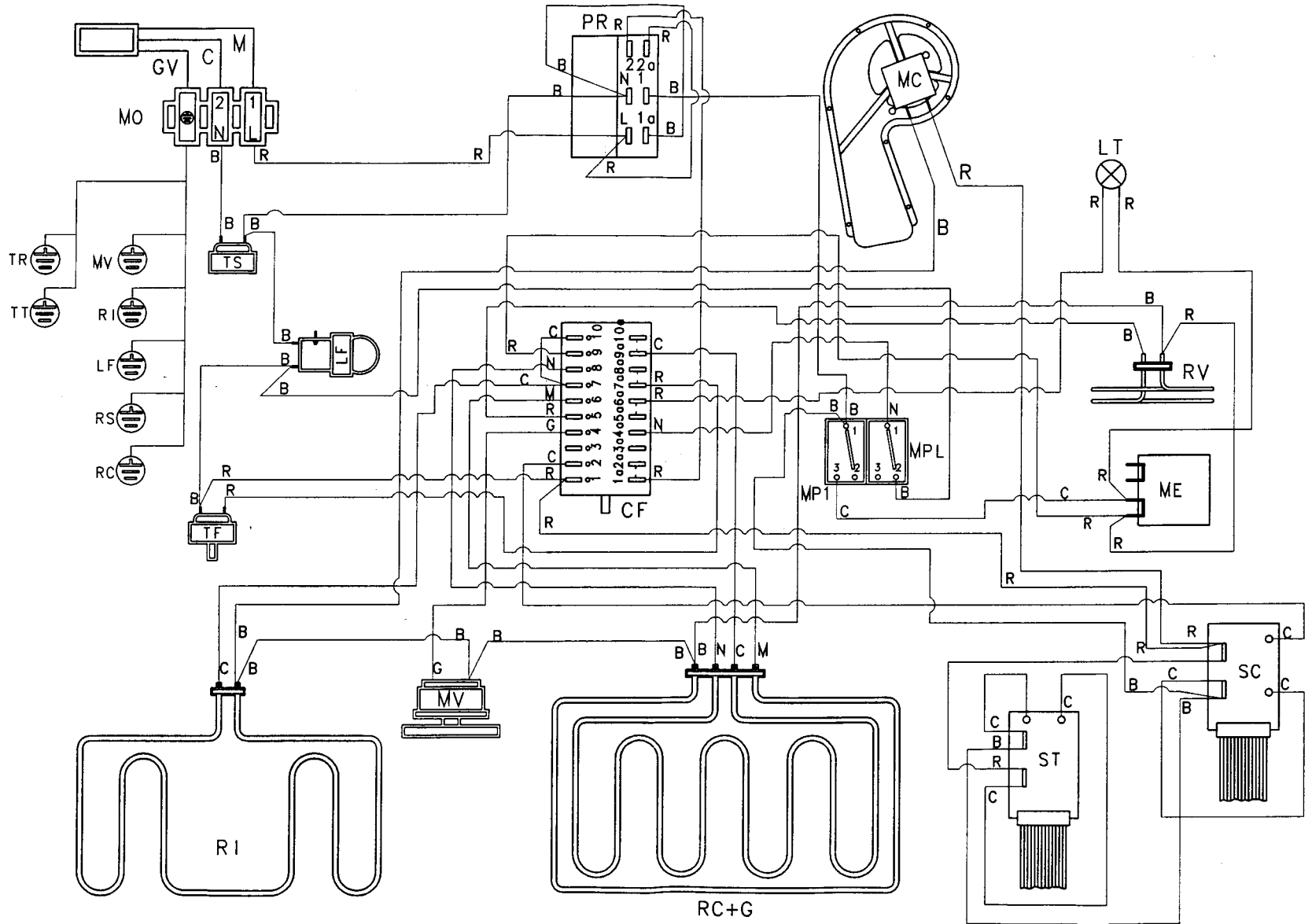
ELECTRIC DIAGRAM PART NUMBER 820731084 MOD.SA650NE
